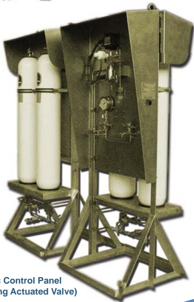
Pneumatic Control Panel (Spring Return Actuated Valve)
